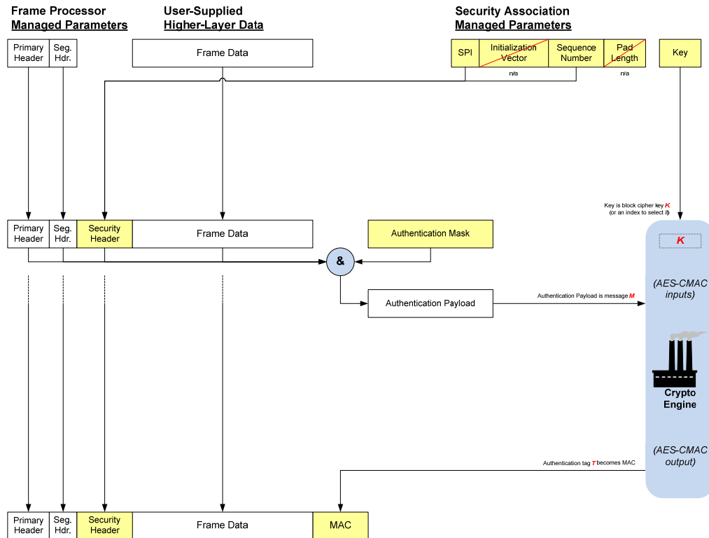
Figure 4-3: TC Authentication (Baseline Implementation)
