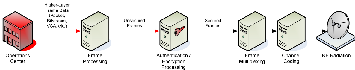
Figure 4-6: Simple Forward Link Scenario (Ground)
