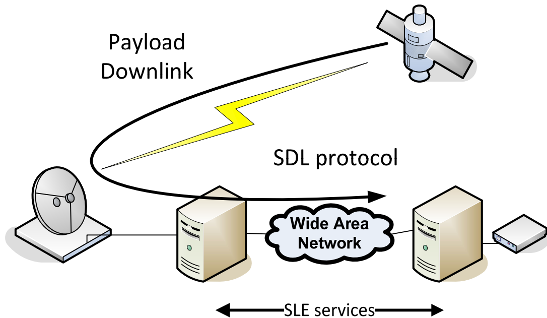
Figure 2-2: Mission Network Topology A
