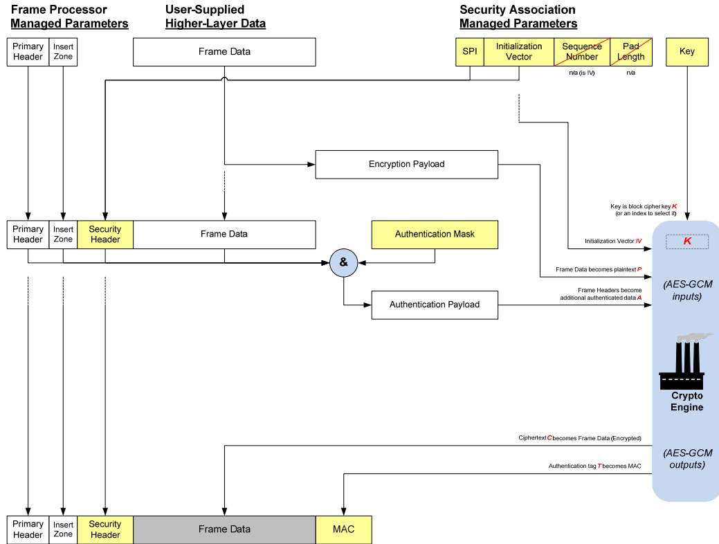
Figure 4-5: AOS Authenticated Encryption (Baseline Implementation)
