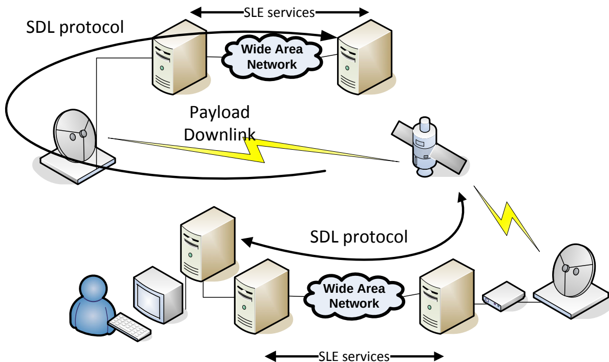
Figure 2-3: Mission Network Topology B
