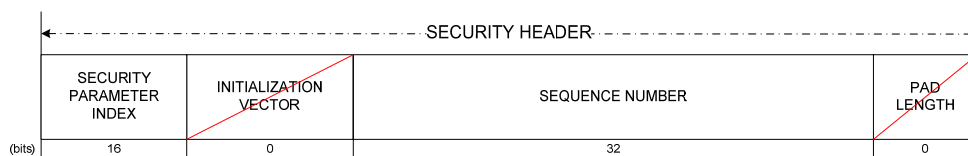
Figure A-1: Security Header (TC Baseline)
