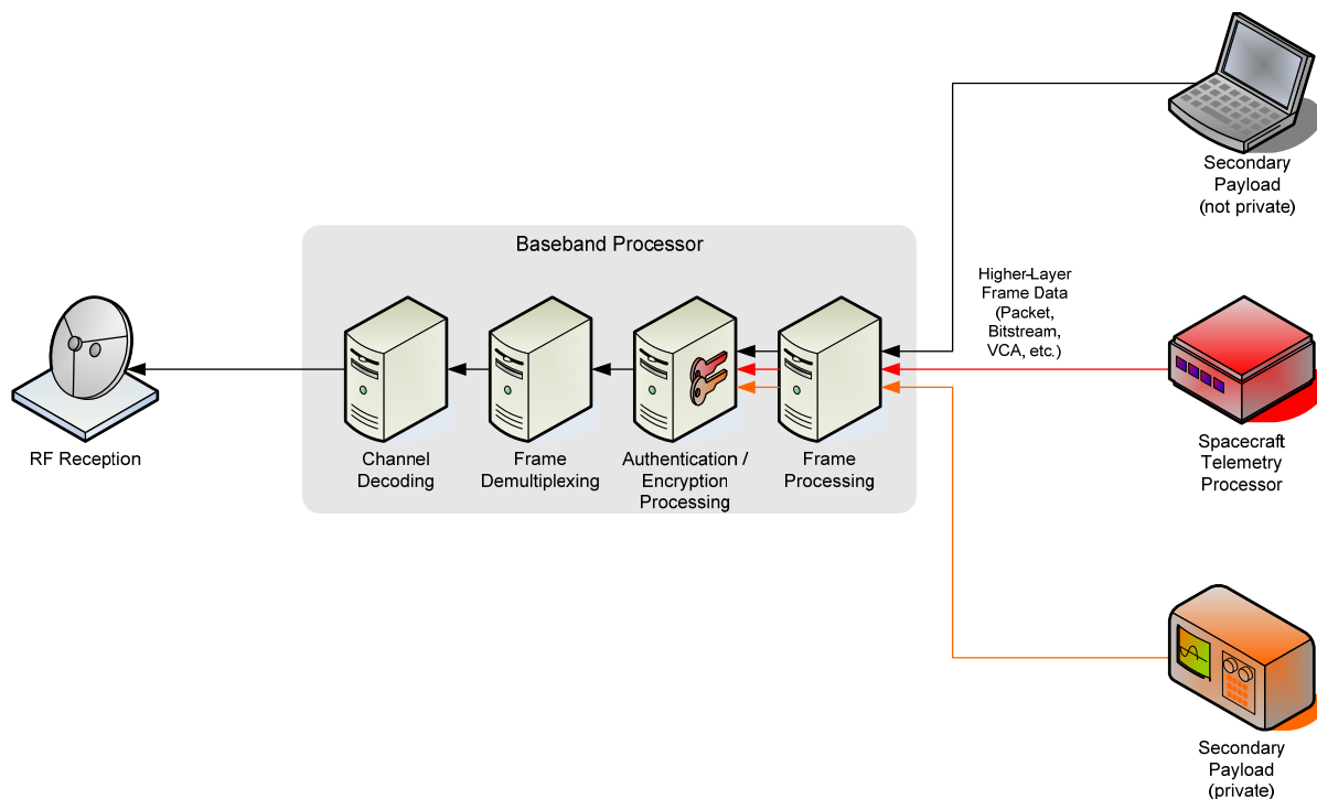
Figure 4-8: Complex Return Link Scenario (Onboard)
