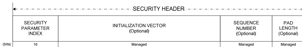
Figure 3-6: Security Header
