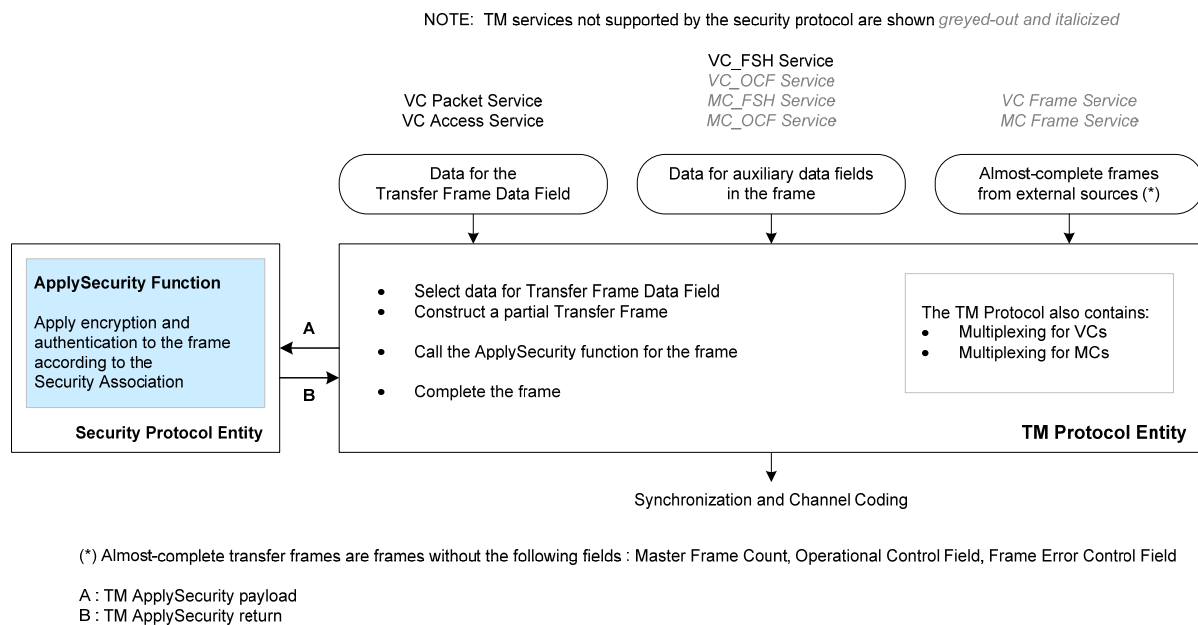
Figure 3-4: Functional Interface within the TM Protocol
