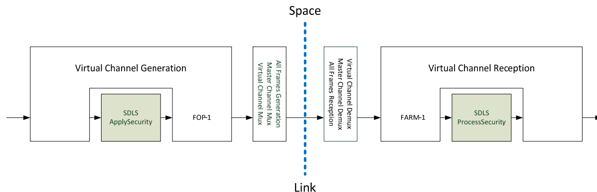
Figure 3-3: Conceptual Interface with the TC SDL Functions
