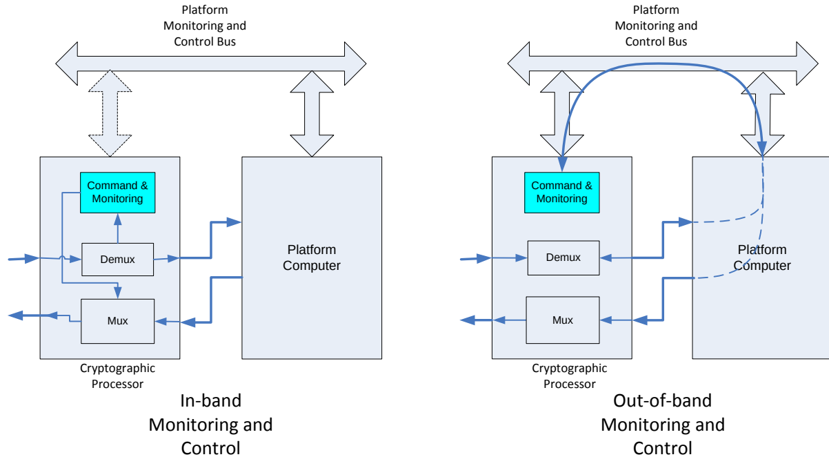
Figure 3-7: Monitoring and Control Options
