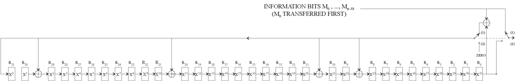
Figure C-1: A Possible Implementation of Encoder
