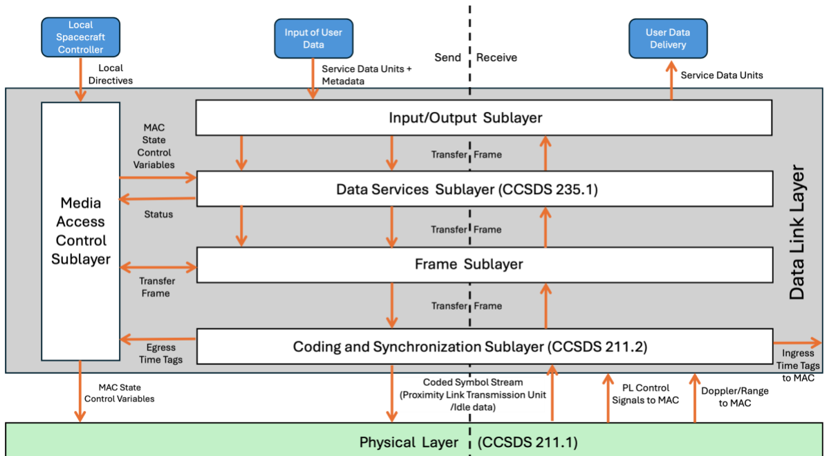
Figure 2-1: Overview of Proximity-1 Layers/Sublayers
