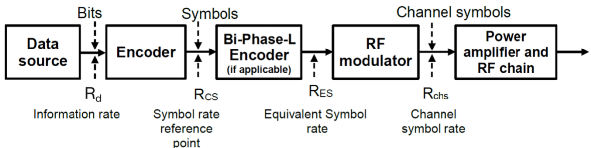
Figure 1-2: Proximity-1 Rate Terminology
