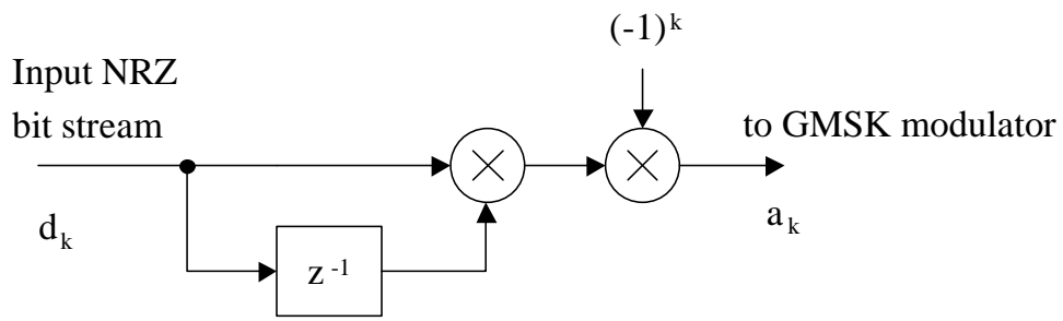
Figure 2.4.17A-1: GMSK Precoder
