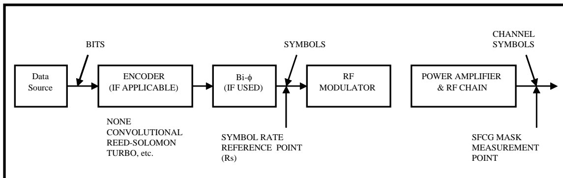
Figure 3.1.2B-2: Symbol Rate Definition
