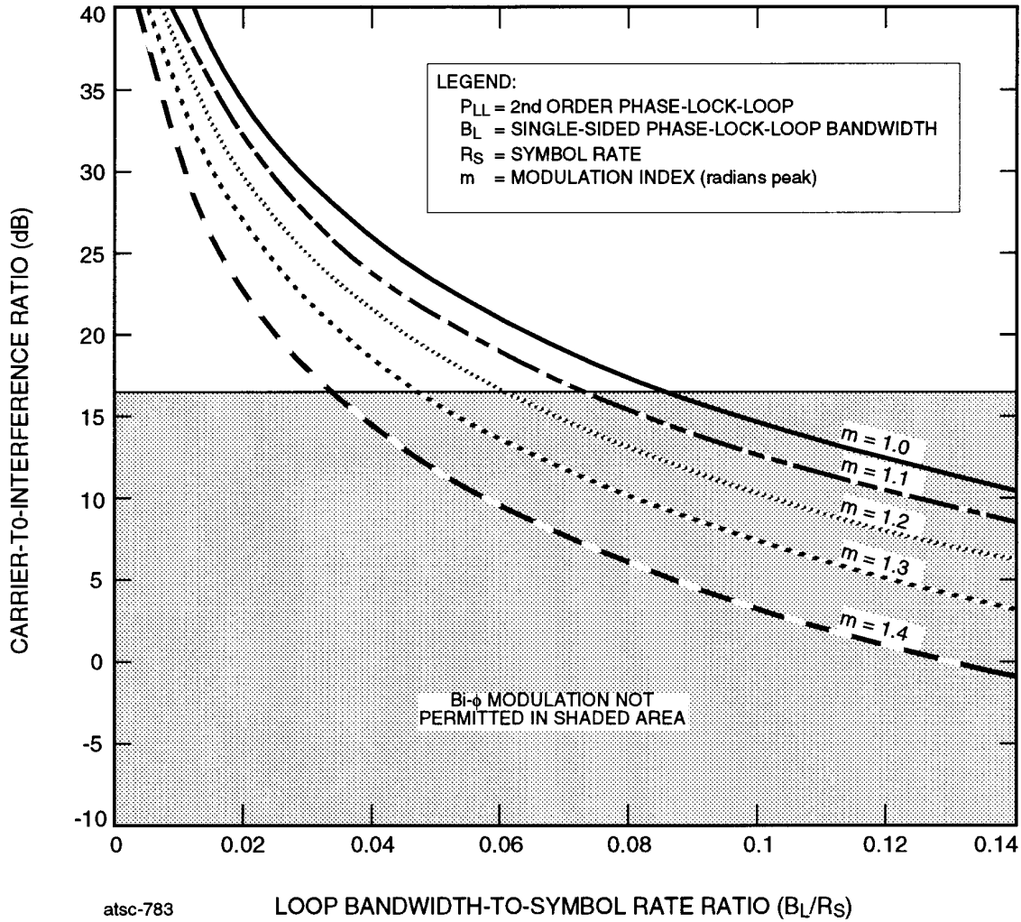
Figure 2.4.15B-1: Operating Region for Use of PCM/PM/Bi- \phi Modulation When No Coding Is Employed
