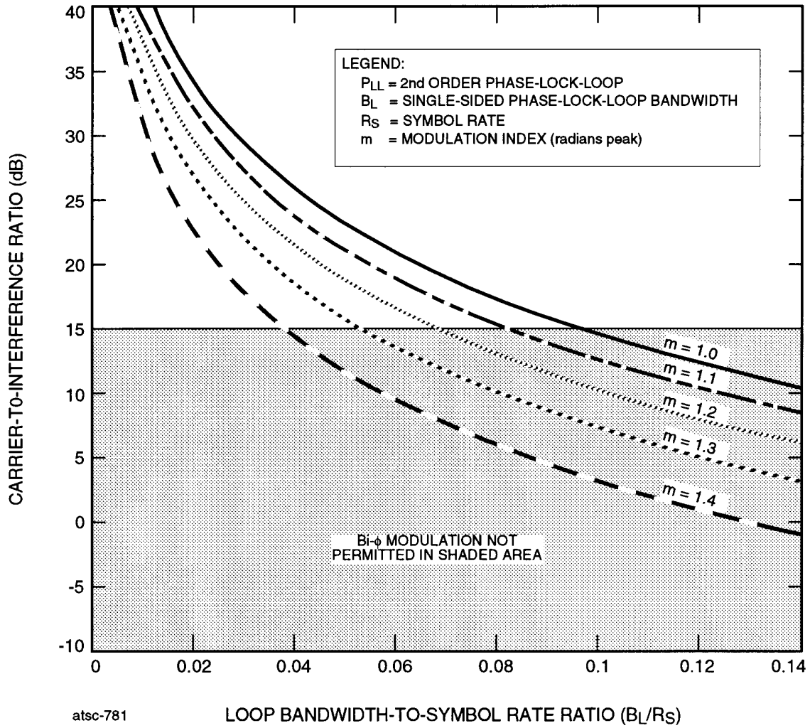
Figure 2.4.15A-1: Operating Region for Use of PCM/PM/Bi- \phi Modulation When No Coding Is Employed
