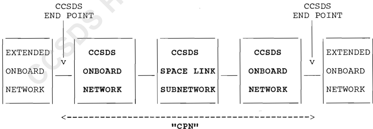
(B) SPACE/SPACE CONFIGURATION
