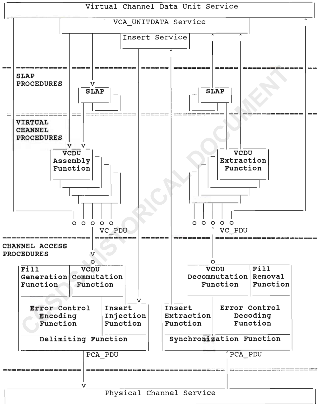
FIGURE 5-9: VCA INTERNAL FUNCTIONAL ORGANIZATION
