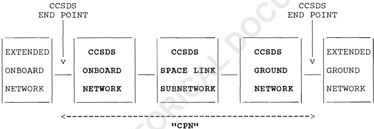
(A) SPACE/GROUND CONFIGURATION
