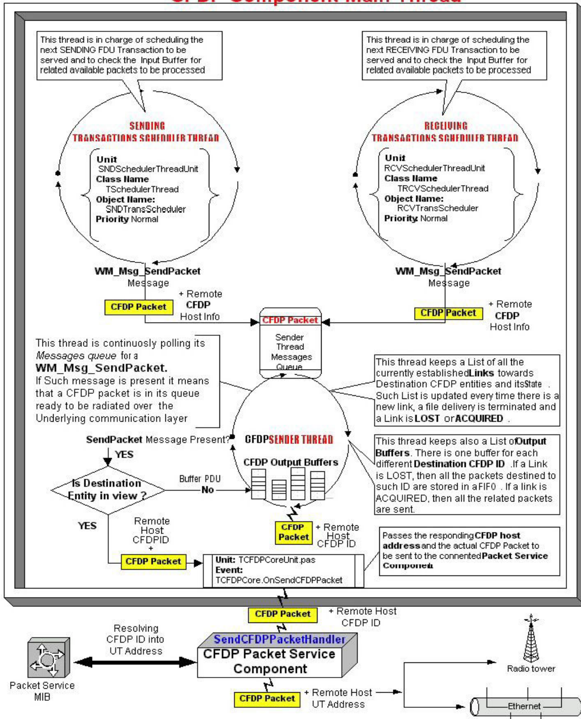
Figure 8-13: CFDP Packets Output Flow Diagram
