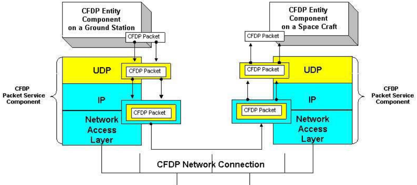
Figure 8-9: CFDP Packet Encapsulation
