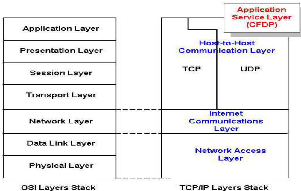
Figure 8-5: Correspondence Between CFDP and OSI Layers
