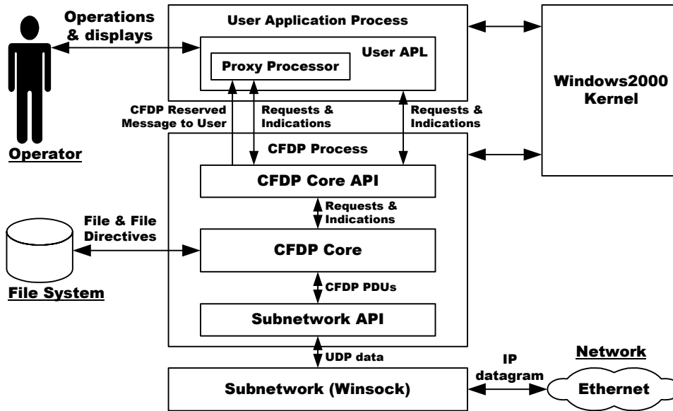
Figure 8-16: The Architecture of NASDA CFDP Implementation
