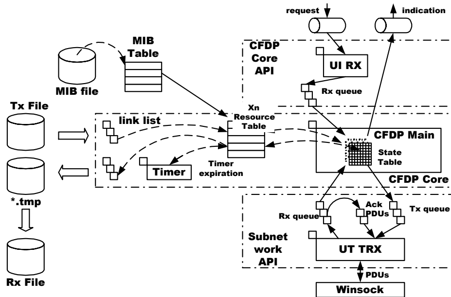
Figure 8-17: CFDP Process
