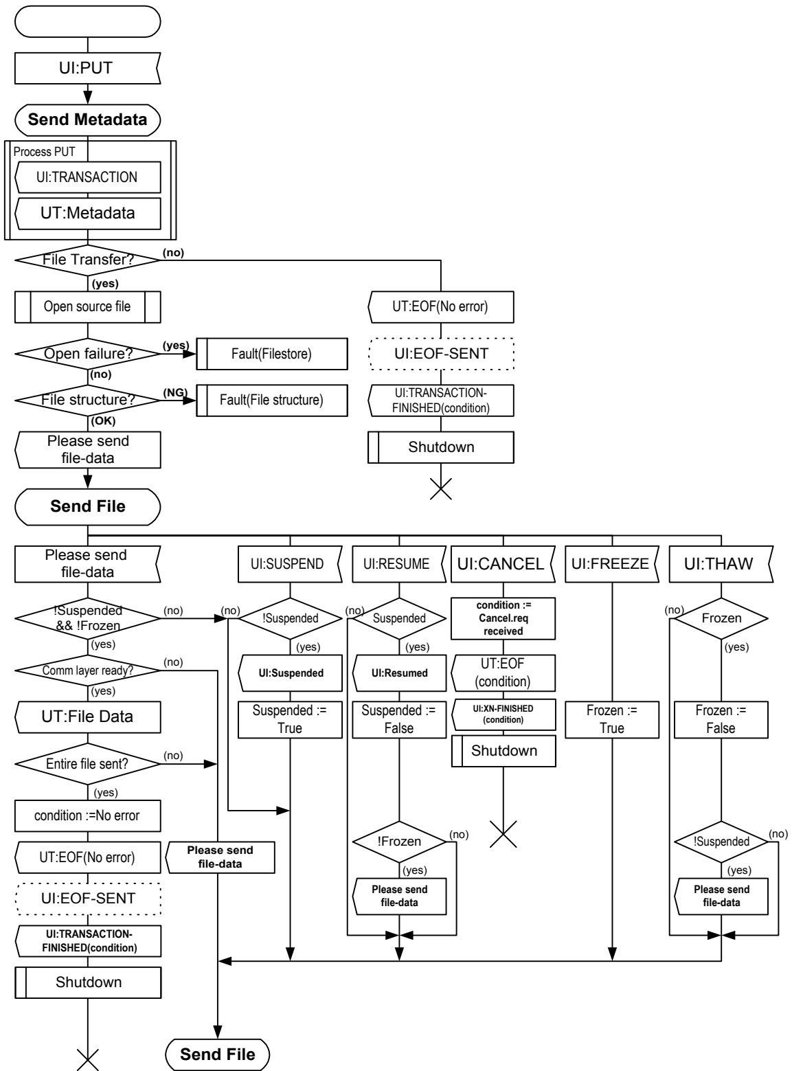
Figure 6-1: Class 1 Source State Diagram
