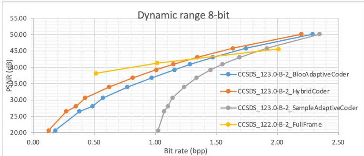
Figure 5-5: Mean PSNR Values of CCSDS Compressors on the 8-bit Test Images
