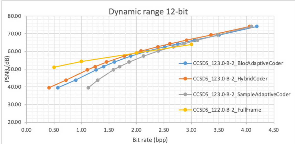
Figure 5-7: Mean PSNR Values of CCSDS Compressors on the 12-bit Test Images
