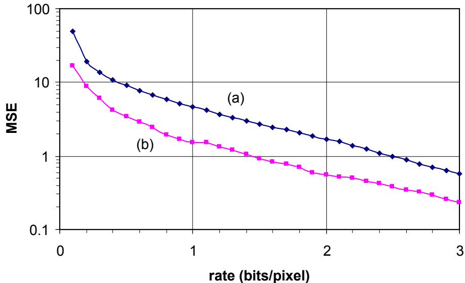
Figure 3-1: Rate Distortion Performance on Transposed Version of coastal_b7 Test Image Using (a) Integer DWT, Fixed-Rate Compression (with UseFill = 1), S = 16 , and (b) Float DWT, Full-Frame ( S = 16384 ) Compression
