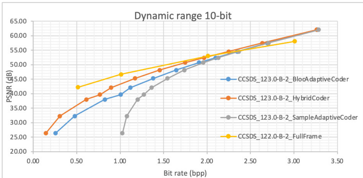
Figure 5-6: Mean PSNR Values of CCSDS Compressors on the 10-bit Test Images
