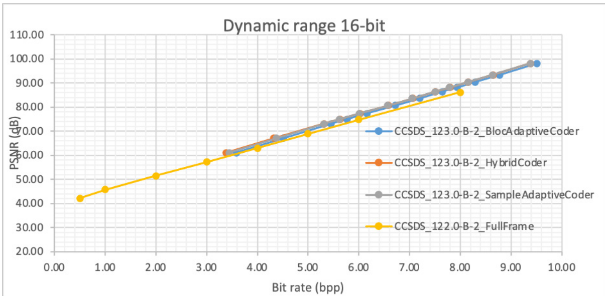
Figure 5-8: Mean PSNR Values of CCSDS Compressors on the 16-Bit Test Images
