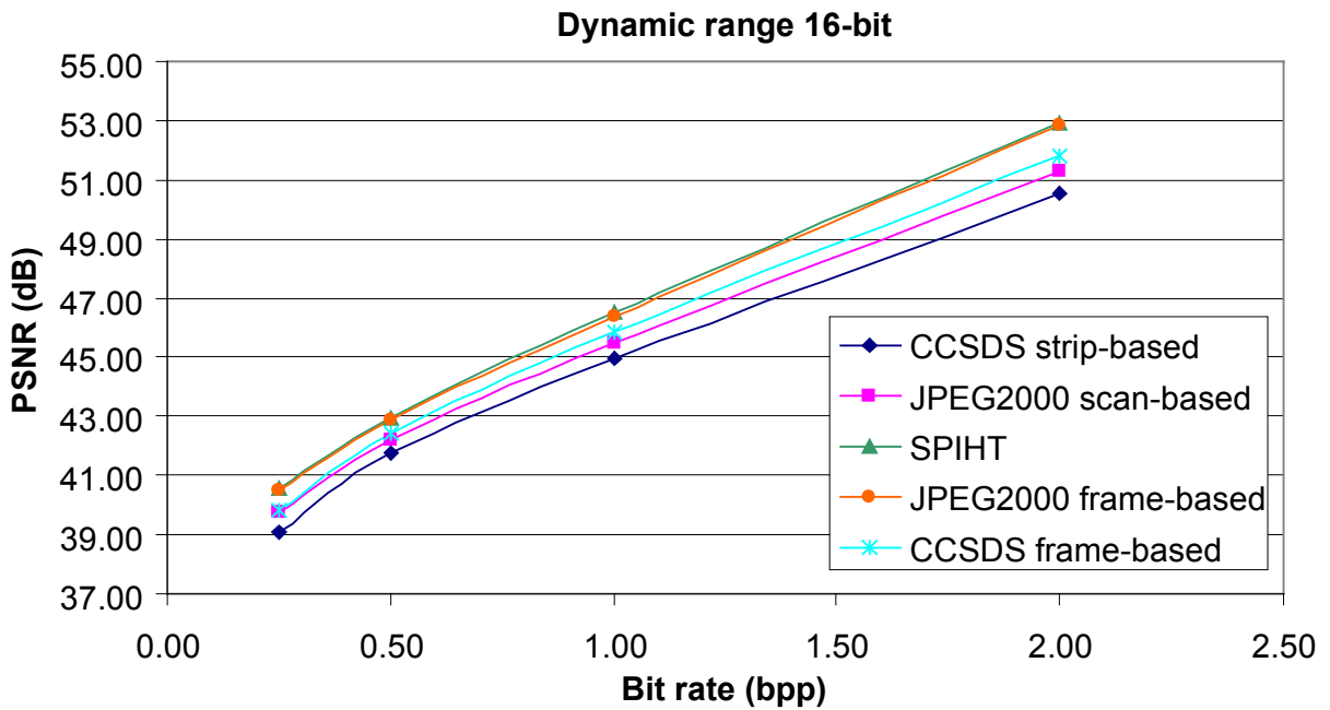
Figure 5-4: Mean PSNR Values for Each Algorithm on the 16-Bit Test Images
