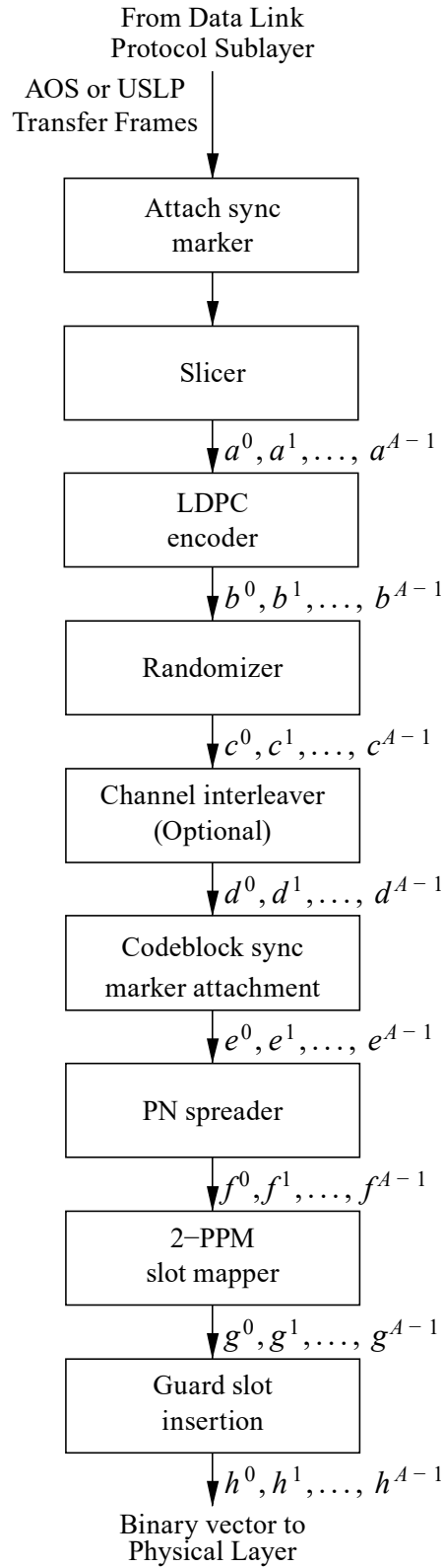
Figure 4-1: Functional Diagram for AOS/USLP Transfer Frame Signaling
