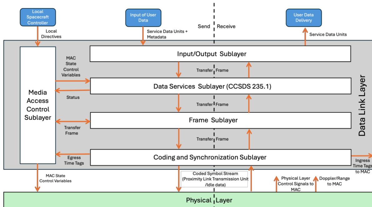
Figure 2-1: Generic Physical and Data Link Sublayers
