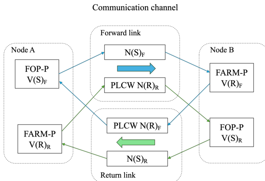
Figure 2-2: COP-P Process
