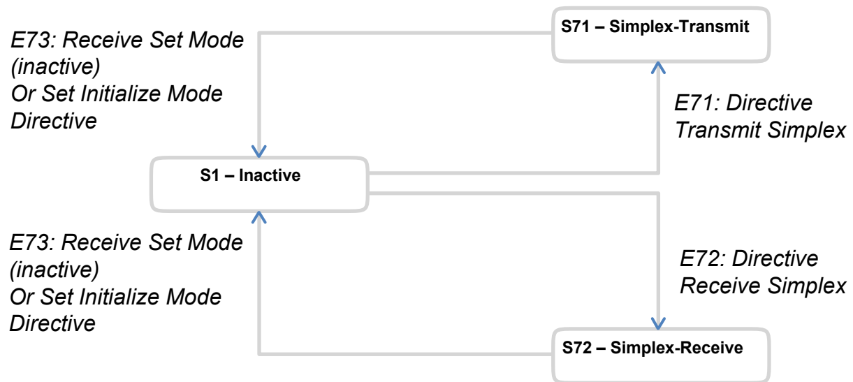
Figure 5-3: Simplex Operations
